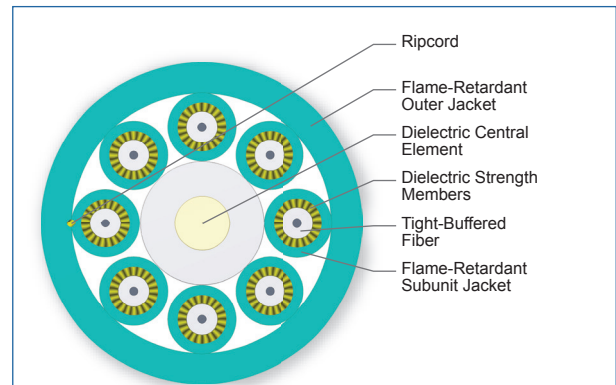
Cross Section of Part Number: 008T61-31391-24
