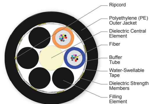
Cross Section of Part Number: 024KN4-T4S30A20
