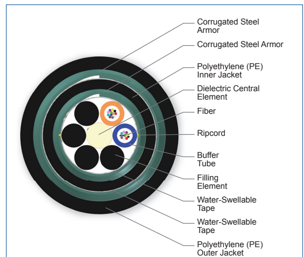
Cross Section of Part Number: 024TUD-T4131D20
