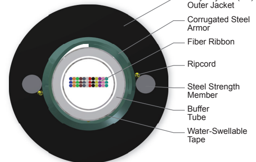
Cross Section of Part Number: 036EC5-14100D53
