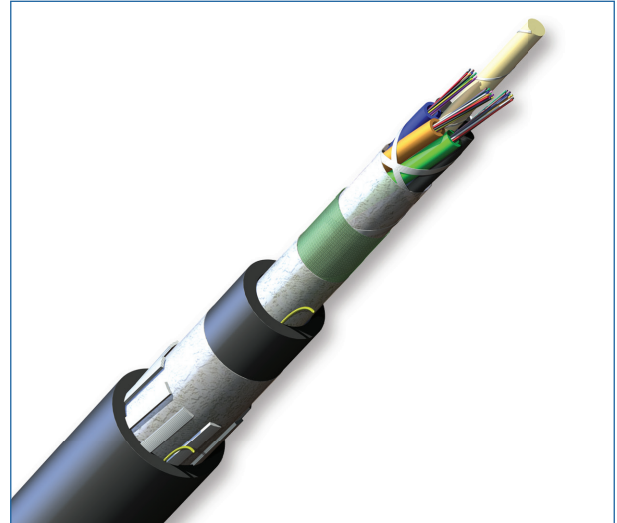
Part Number: 036KUL-T3630D2M
