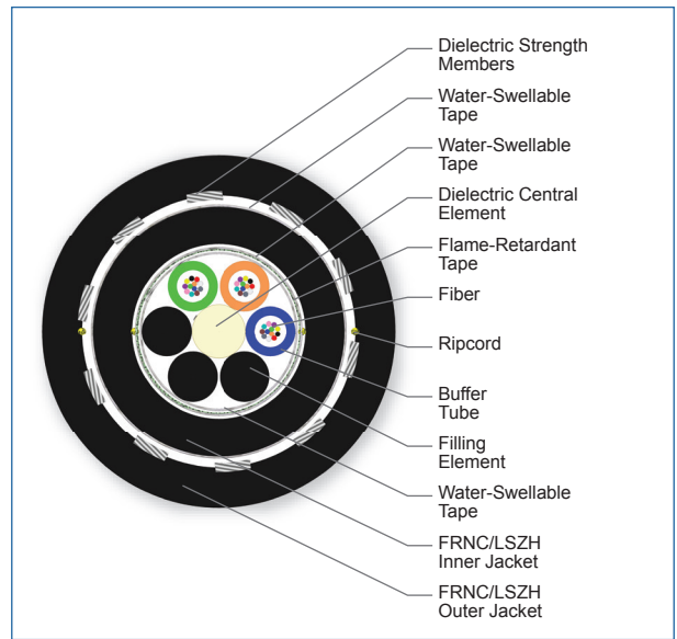
Cross Section of Part Number: 036KUL-T3630D2M
