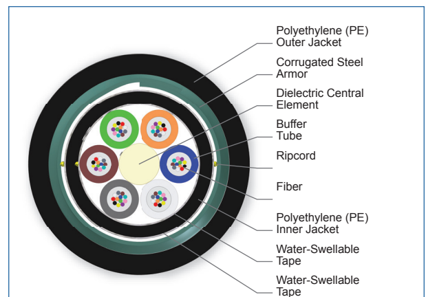
Cross Section of Part Number: 072EU5-T4101C20
