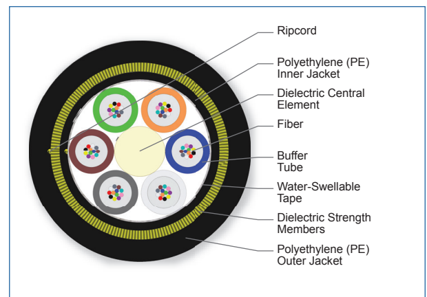
Cross Section of Part Number: 072TAE-T4531A20
