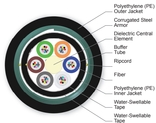
Cross Section of Part Number: 072TU5-T4131C20
