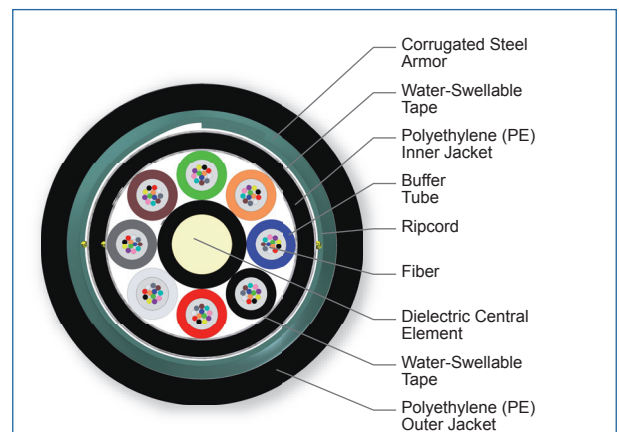
Cross Section of Part Number: 096EU5-T4101C20
