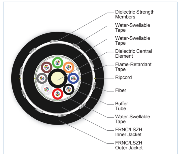
Cross Section of Part Number: 096KUL-T3630D2M
