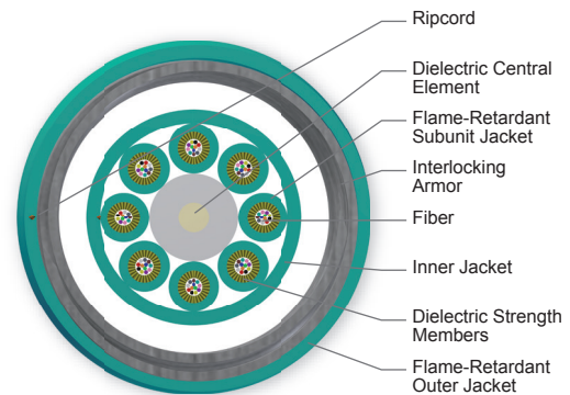
Cross Section of Part Number: 096TD8-T1390-A3
