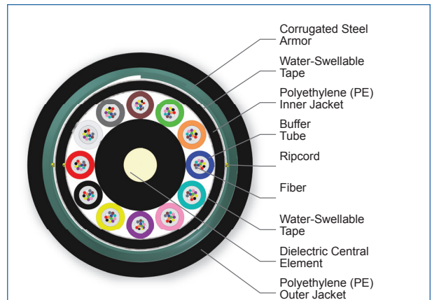
Cross Section of Part Number: 144EU5-T4101C20
