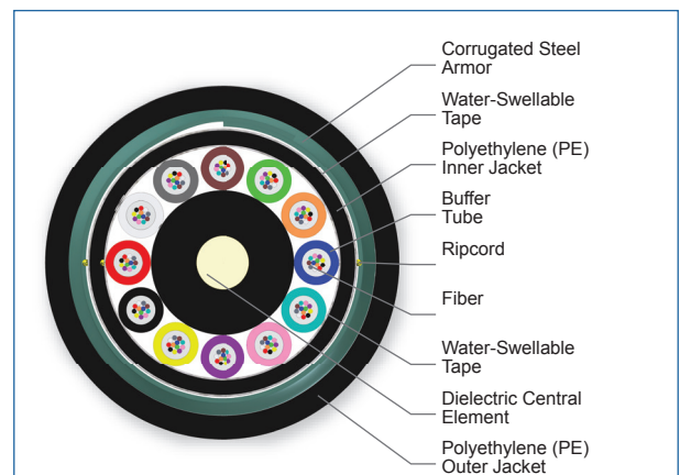
Cross Section of Part Number: 144KU5-T4130C20
