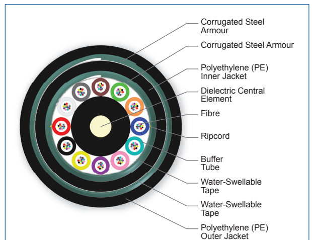
Cross Section of Order Number: 144TUD-T4131D20
