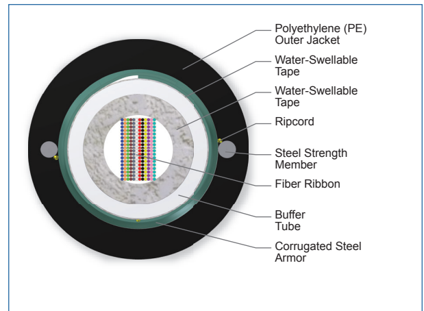
Cross Section of Part Number: 216EC5-14100D53
