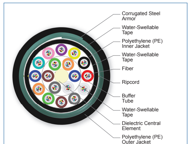
Cross Section of Part Number: 216TU5-T4131C20
