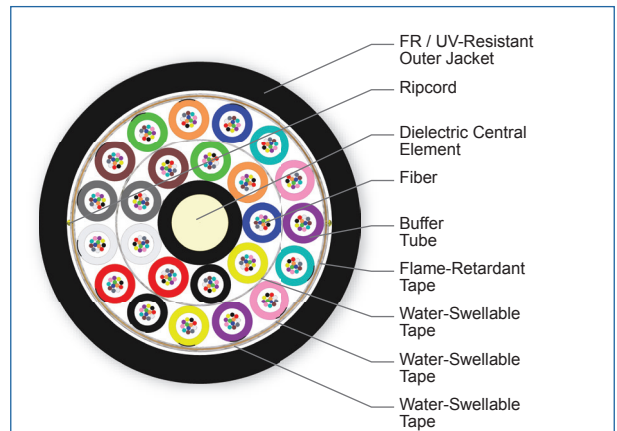
Cross Section of Part Number: 288TUF-T4131D20
