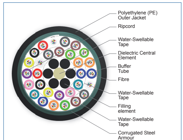
Cross Section of Order Number: 360EUC-T4101A20
