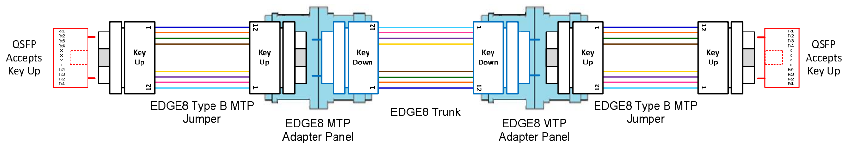
Figure 10-a: Parallel Connectivity Utilizing an 8-fiber Type B MTP® Jumper
