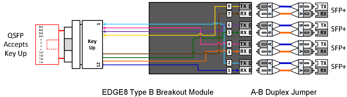
Figure 16-a: 8-fiber to 2-Fiber Inter-connect Structured Cabling Utilizing a Port Breakout Module
