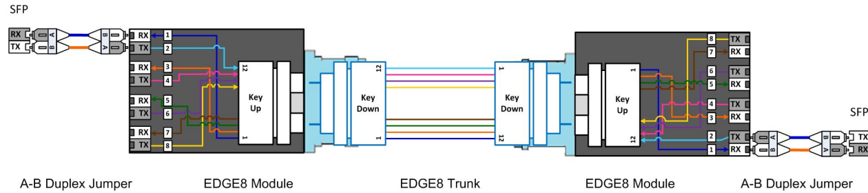
Figure 7-a: Duplex Connectivity with Inter-connect Structured Cabling
