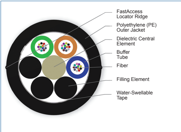
ALTOS All-Dielectric Cable with FastAccess Technology, Gel-Free, 36 Fibers | Photo PIM2326
