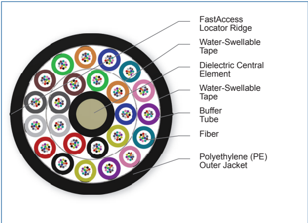
ALTOS All-Dielectric Cable with FastAccess Technology, Gel-Free, 288 Fibers | Photo PIM2334
