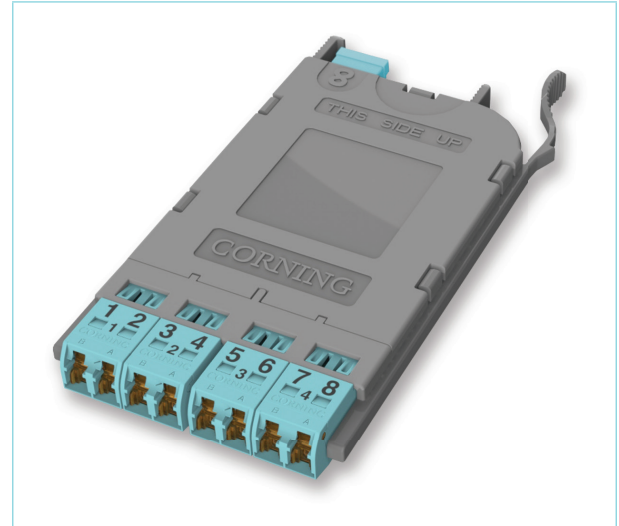
EDGE8 MTP to LC Duplex Module | Photo REN389
