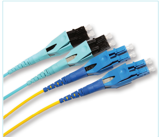
Reverse Polarity Uniboot Duplex Patch Cords | Photo LAN2223
