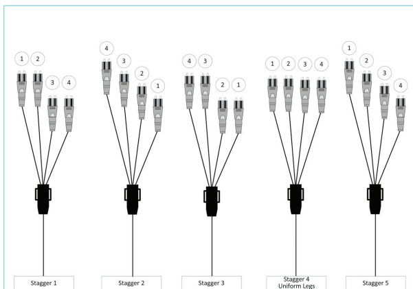
EDGE8 Staggered Harness Examples | Photo ZA4253
