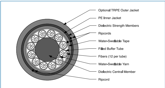
SOLO Cable, 144-Fiber | Drawing ZA-1950
