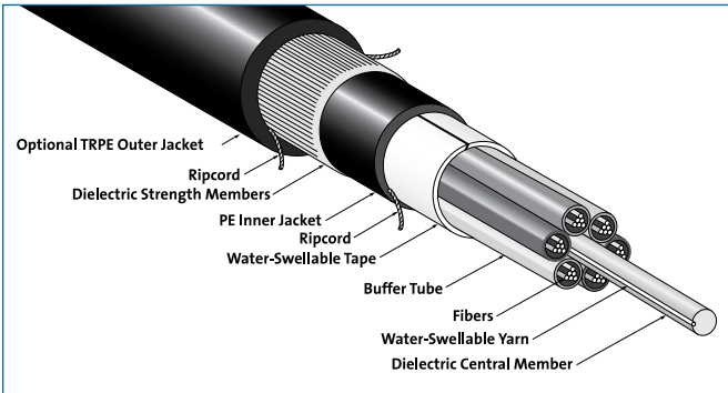
SOLO ADSS Cable | Drawing ZA-1948
