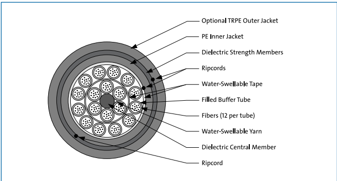
SOLO Cable, 216-Fiber | Drawing ZA-1951
