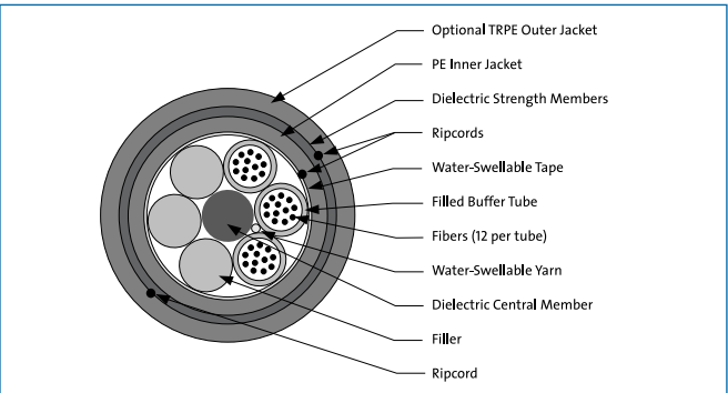
SOLO Cable, 36-Fiber | Drawing ZA-1949
