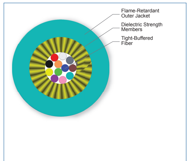
MIC 250 Interconnect Cables, 12 Fibers | Photo PIMtbd
