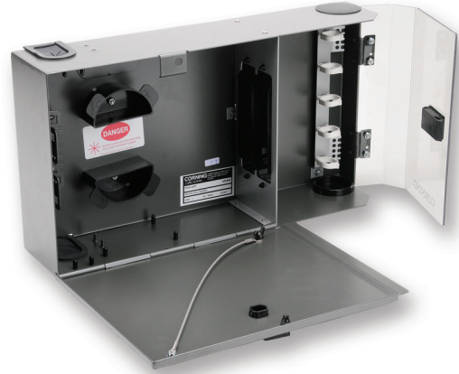
Pretium Wall-Mountable Housing (PWH) | Photo LAN763
